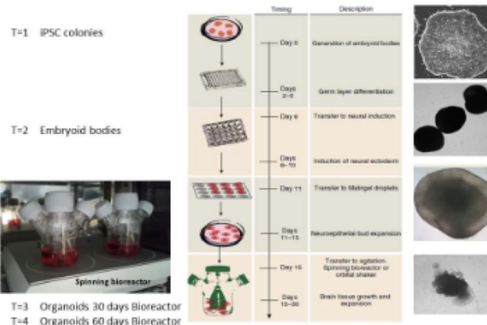
Figure 1: Schematic representation of the generation of FOXP1 mutant organoids
